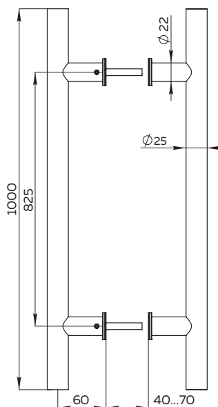
PULL.PH25/825.22 INOX 304
