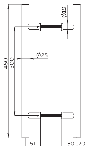
PULL.PH25/300.22 INOX 304
